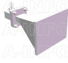
LB-90-15-C-TFSPO Standard Gain Horn Antenna 8.2-12.4GHz 15dB Gain TNC Female
